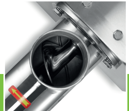
Worm gear and screw ring in stainless steel
