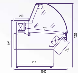
Vidros Curvos / Curved Glass Vitres Arrondis / Cristales Curvos
