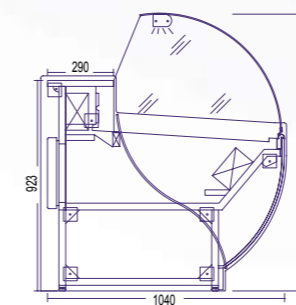
Vidros Curvos / Curved Glass Vitres Arrondis / Cristales Curvos
